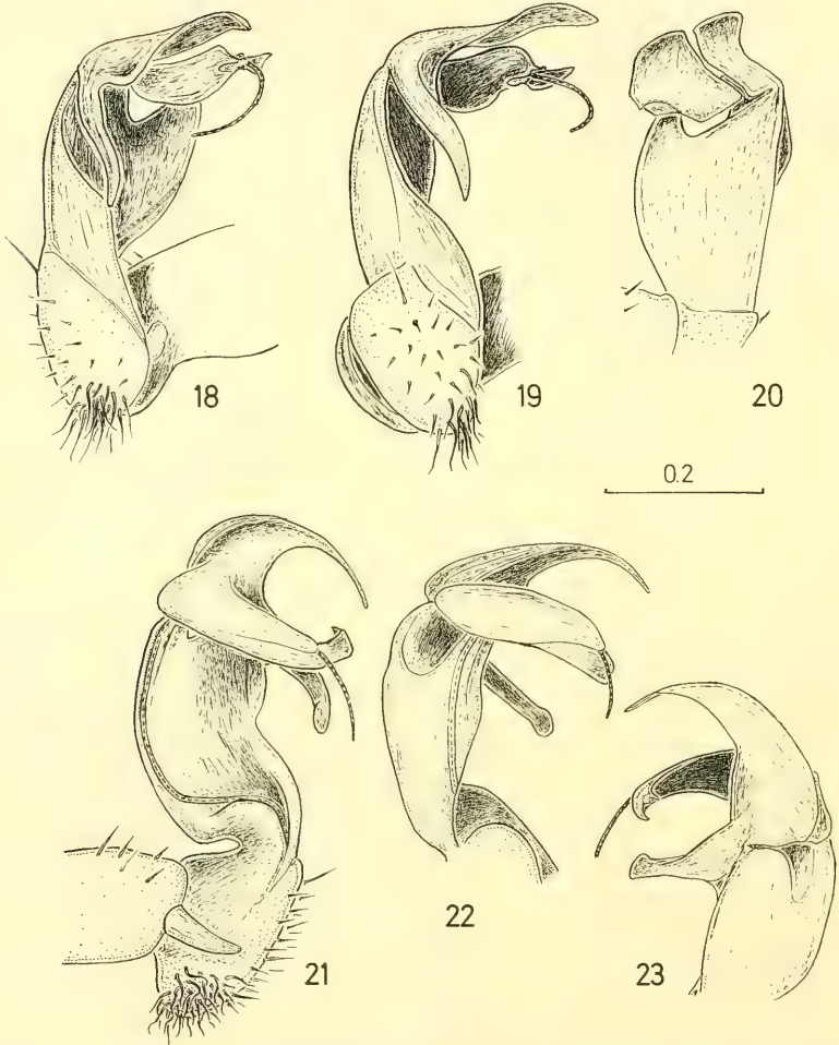
Figs 18–23. Gonopods of Paraneddyopus cylindricus (Carl, 1935); ♂♂ from Gitang Khola (18–20) and Mt. Phulchoki (21–23), respectively (ventromesal, ventral, lateral, mesal, dorsal and ventral views, respectively).
